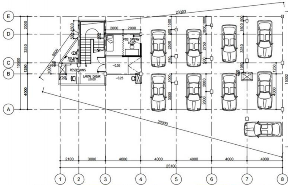
Denah Lantai 1
