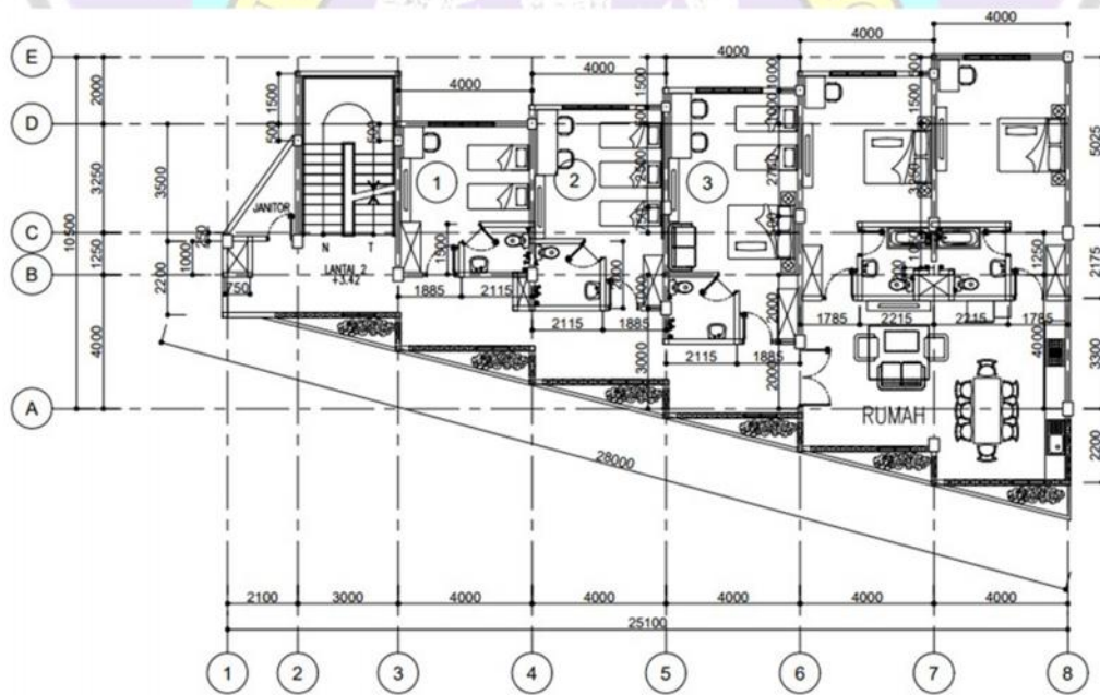
Denah Lantai 2
